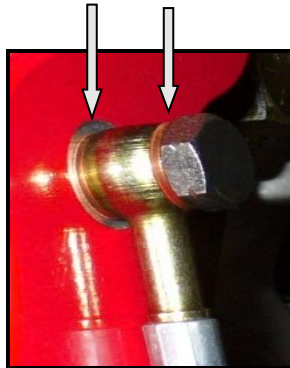
Figure 7: Stainless steel braided brake hose installed to the caliper
